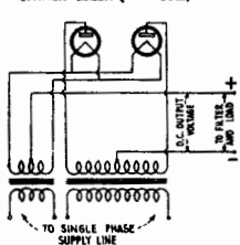
SINGLE PHASE FULL-WAVE RECTIFIER CIRCUIT (TWO TUBES)
